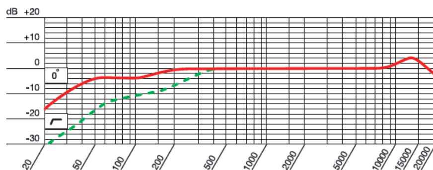
Frequency Response
