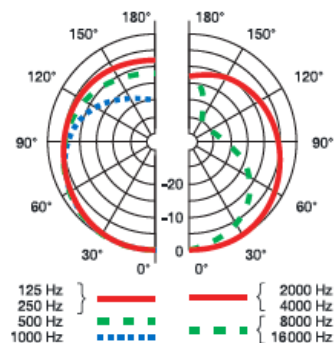
Polar Diagram
